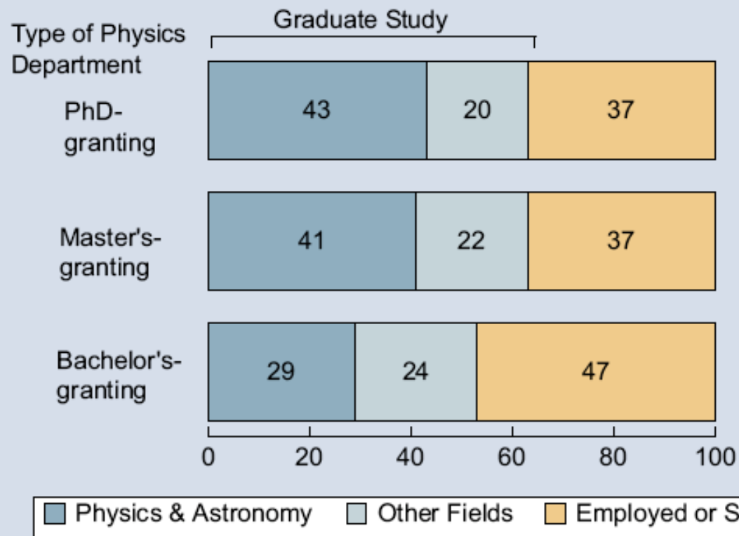
Figure 4. Initial outcomes by type of department attended, physics bachelor's classes of 2003 & 2004.
